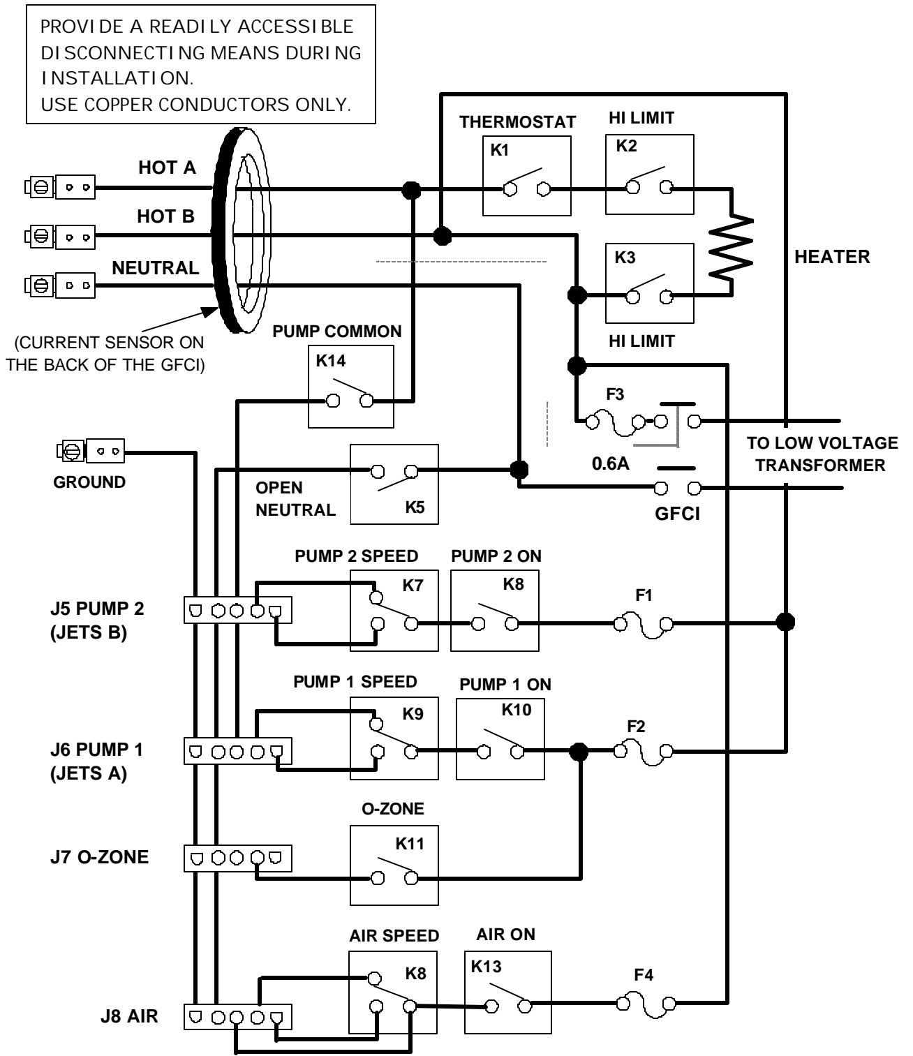
P1PC-G39 AC WIRING
