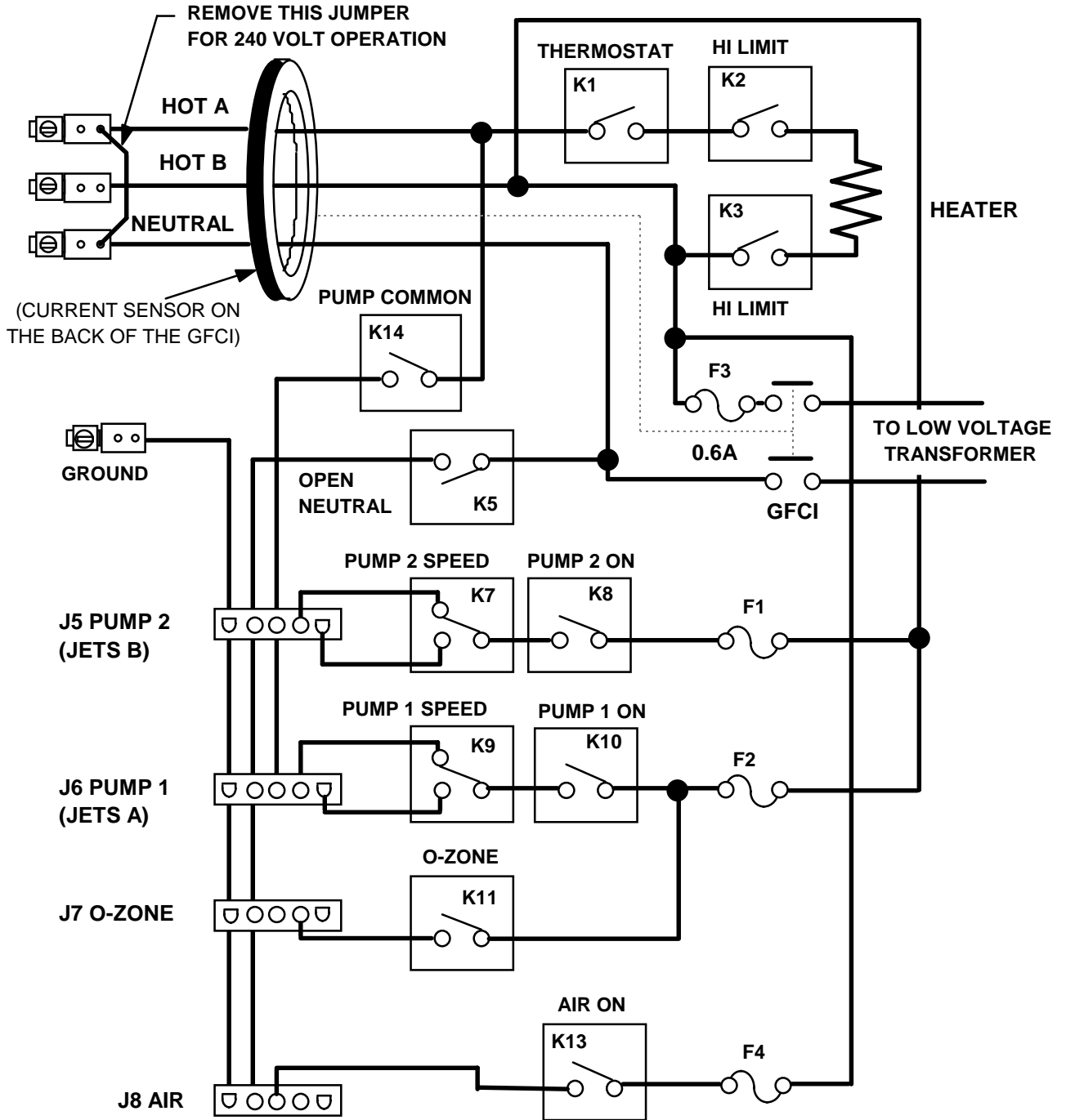
P1MC/P2MC-G38 AC WIRING
